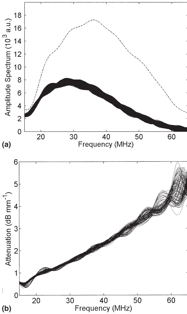
Fig. 3. Attenuation measurements (a) Plot of the mean amplitude spectrum from the reference well (dotted line) and an overlay of 30 scan lines of the mean amplitude spectra for different locations in the pellet well containing HEK cells. (b) Plot of \alpha(\nu) , in \text{dB mm}^{-1} , corrected for water attenuation. The frequencies used in the analysis were from 20 to 60 MHz, corresponding to the relevant transducer bandwidth.
