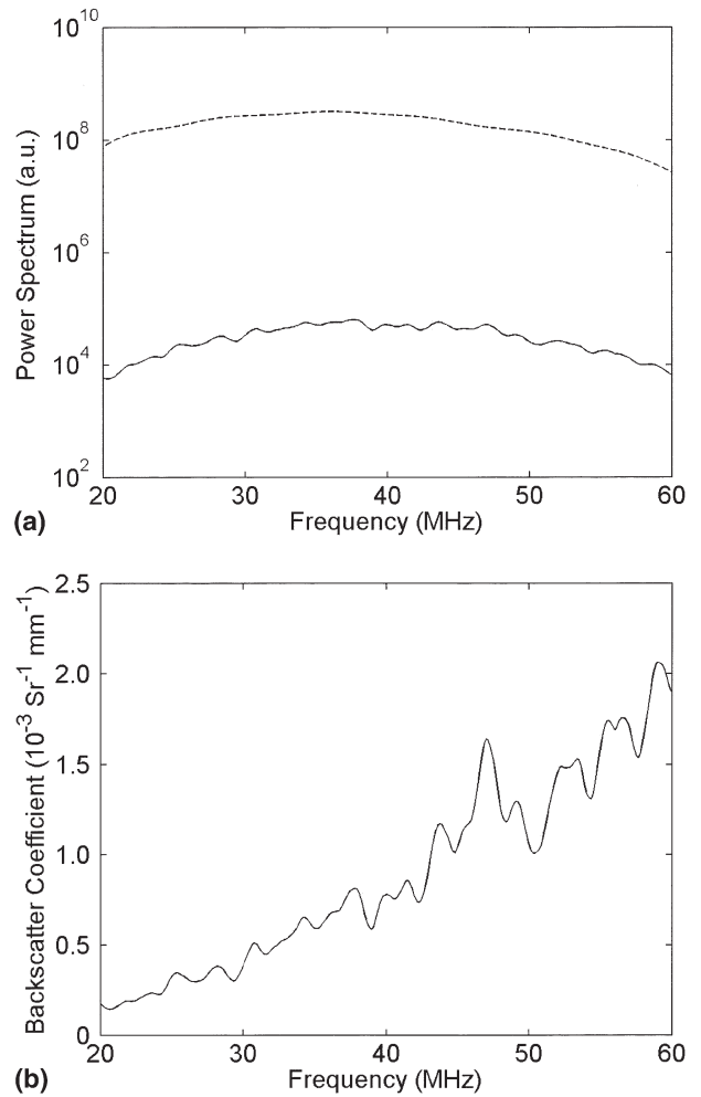
Fig. 4. Backscatter measurements (a) Plot of the mean power spectrum from the reference well (dotted line) and the ROI of the HEK cell pellet (solid). (b) Calculated backscatter coefficient as a function of frequency. The frequencies used in the analysis were from 20 to 60 MHz, corresponding to the relevant transducer bandwidth.
